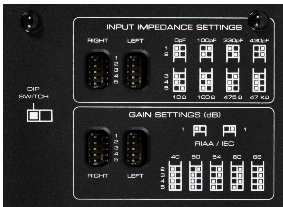
Figure 2: The 110LP v2 cartridge adjustments
