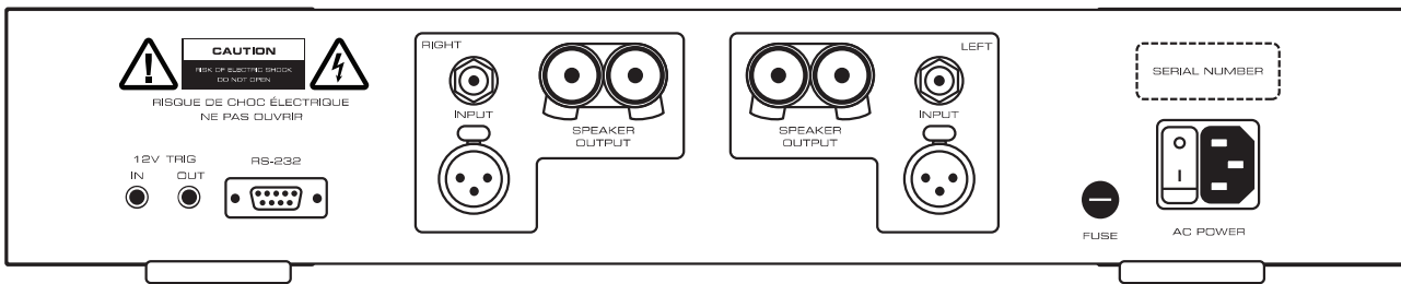
Figure 1: 330A Backpanel
