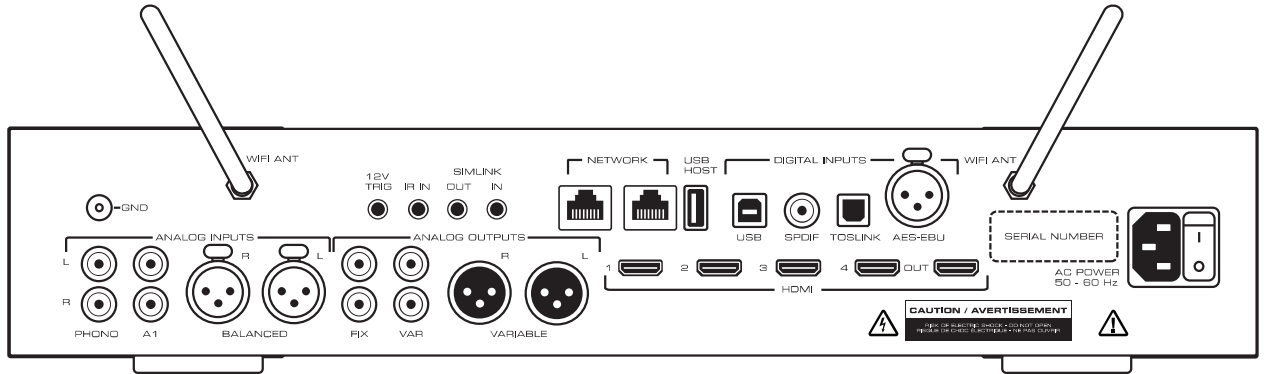
Figure 2: 390 Backpanel
