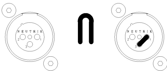
Figure 2: XLR connector without and with jumper accessory
