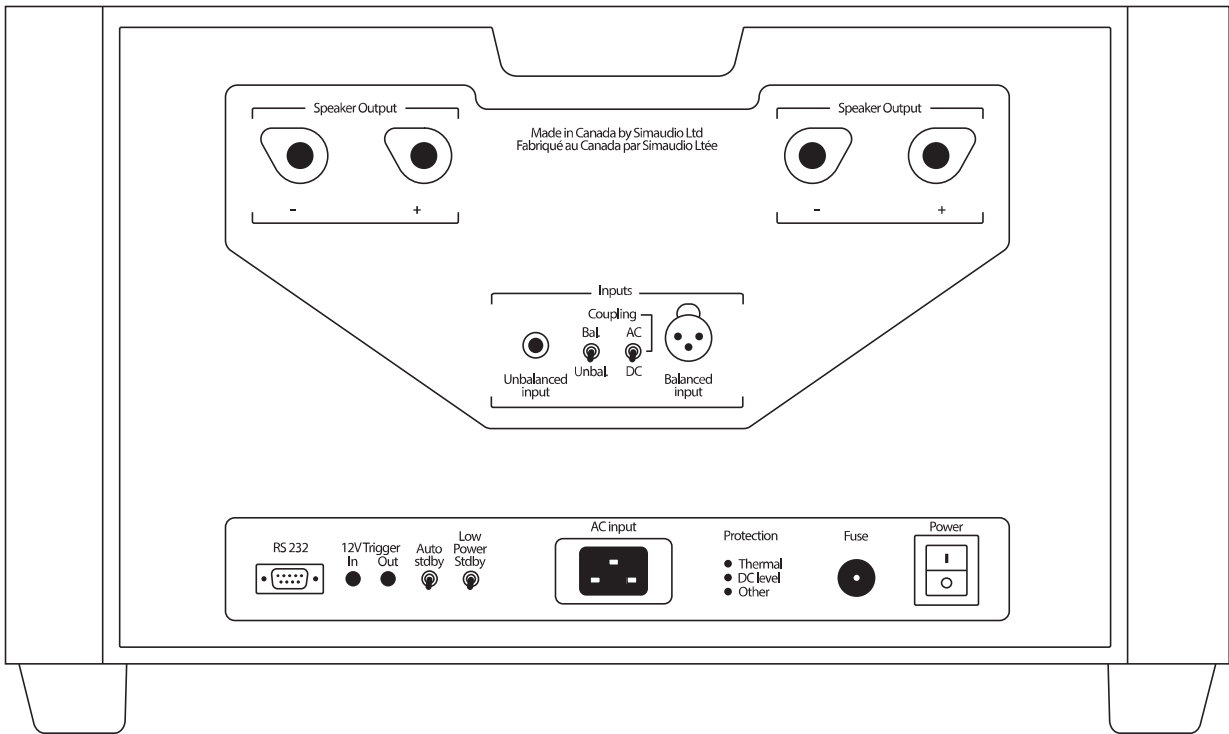
Figure 1: 888 Backpanel
